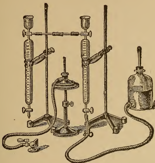
Fig. 103. APPARATUS FOR MEASURING VOLUME OF HYDROGEN.
